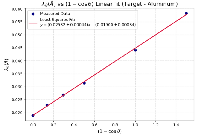
FIG. 9. Linear fit of the measured wavelength shift \lambda_\theta versus (1 - \cos \theta) used to determine the Compton wavelength using Aluminum target.
