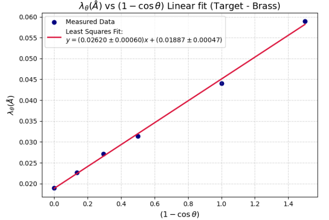
FIG. 10. Linear fit of \lambda_\theta versus (1 - \cos \theta) for the brass target
